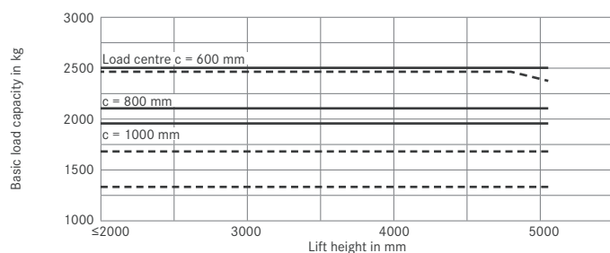
RX 70-25/600 telescopic mast/HiLo mast Single superelastic tyres
