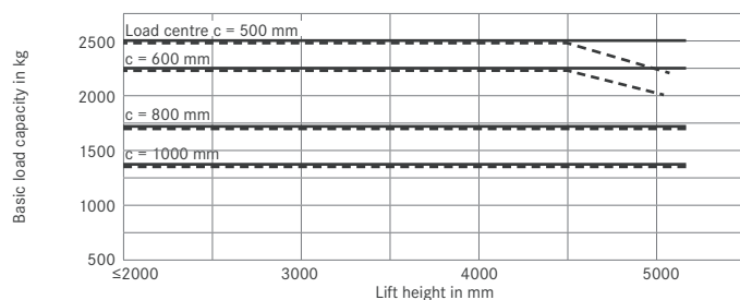
RX 70-25 telescopic mast/HiLo mast Single superelastic tyres
