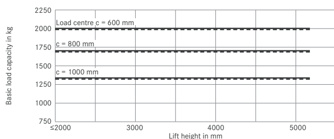
RX 70-20/600 telescopic mast/HiLo mast Single superelastic tyres
